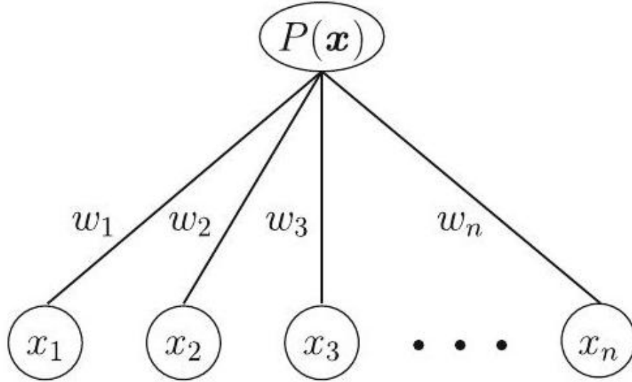
Figure 9.9: Graphical representation of a perceptron as a two-layer neural network
