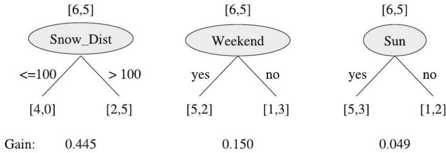
Figure 9.23: The calculated gain for the various attributes reflects whether the division of the data by the respective attribute results in a better class division. The more the distributions generated by the attribute deviate from the uniform distribution, the higher the information gain
