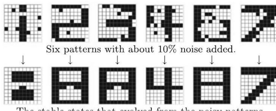
Figure 10.6: For ten learned states the network shows chaotic behavior. Even with little noise the network converges to the wrong patterns or to artifacts
