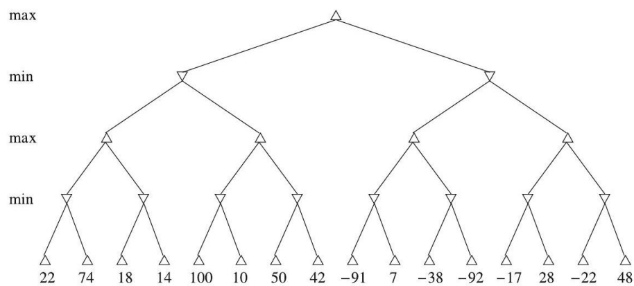
Figure 7.16: Minimax search tree
