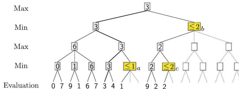
Figure 7.14: A minimax game tree with look-ahead of four half-moves
