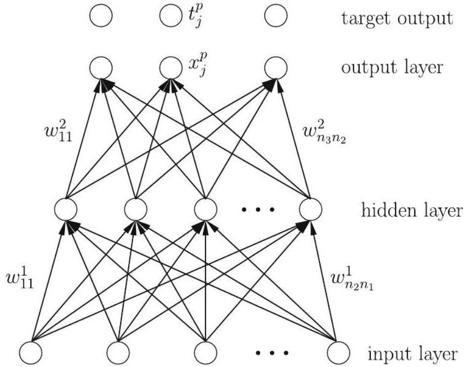
Figure 10.13: A three-layer backpropagation network with n_1 neurons in the first, n_2 neurons in the second, and n_3 neurons in the third layer
