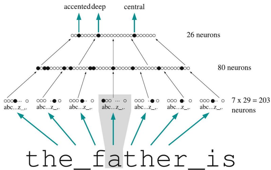
Figure 10.15: The NETtalk network maps a text to its pronunciation attributes
