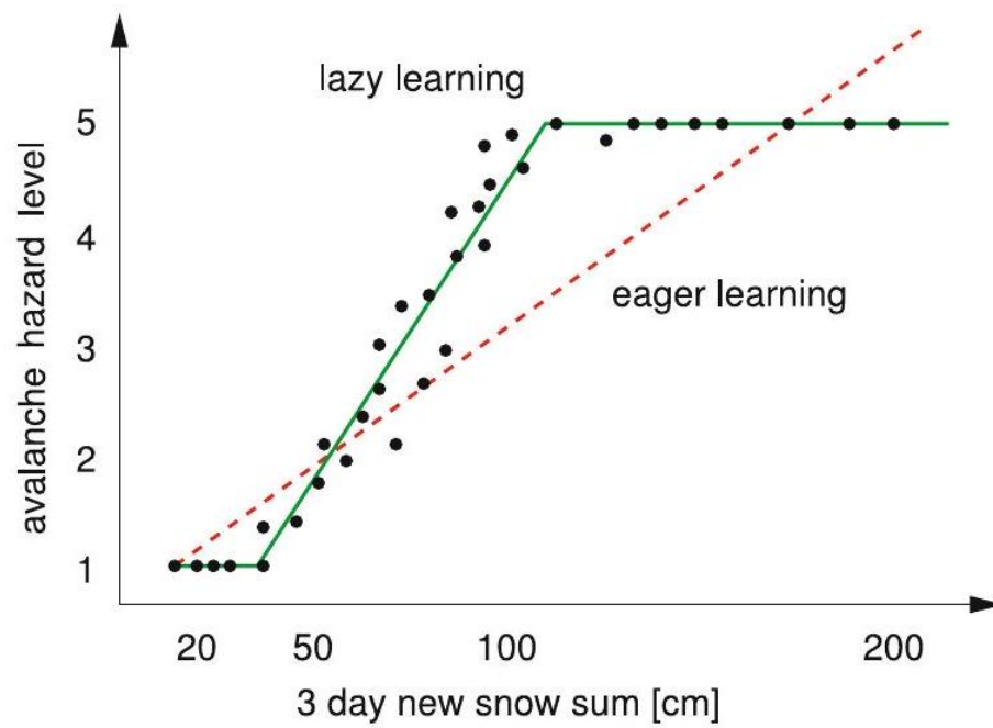
Figure 9.19: To determine avalanche hazard, a function is approximated from training data. Here for comparison are a local model (solid line), and a global model (dashed line)
