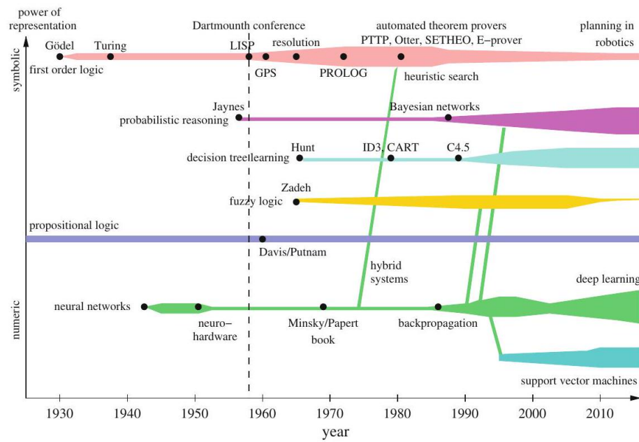
Figure 2.3: History of the various AI areas. The width of the bars indicates prevalence of the method's use
