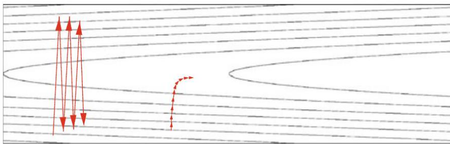
Figure 10.12: Gradient descent for a large \eta (left) and a very small \eta (right) into a valley descending flatly to the right. For a large \eta there are oscillations around the valley. For a \eta which is too small, in contrast, convergence in the flat valley happens very slowly
