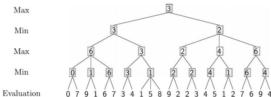
Figure 7.13: A minimax game tree with look-ahead of four half-moves
