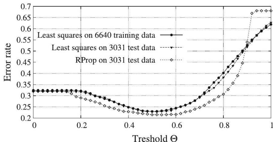
Figure 10.11: Least squares error for training and test data
