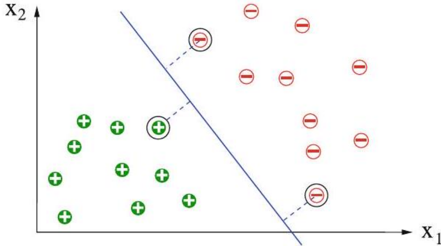
Figure 10.19: Two classes with the maximally dividing line. The circled points are the support vectors
