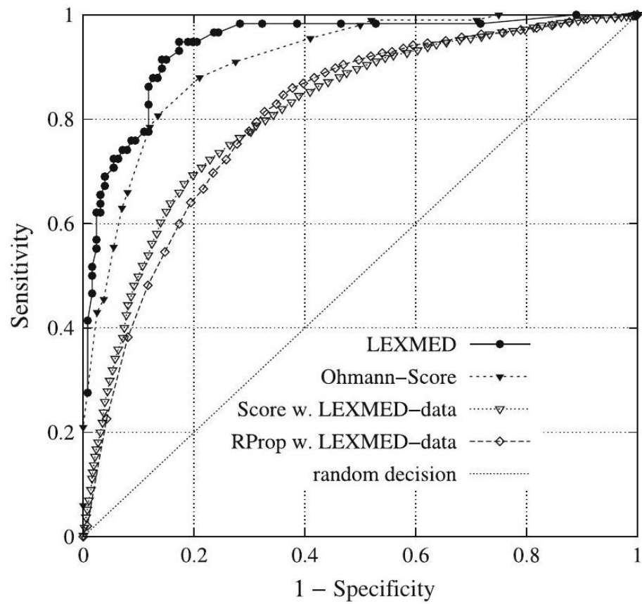
Figure 8.7: ROC curve from Lexmed compared with the Ohmann score and two additional models
