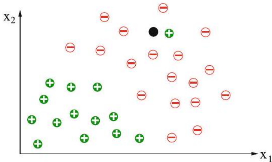
Figure 9.15: The nearest neighbor method assigns the new point marked in black to the wrong (positive) class because the nearest neighbor is most likely classified wrong
