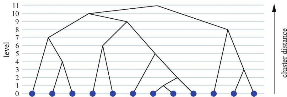
Figure 9.32: In hierarchical clustering, the two clusters with the smallest distance are combined in each step
