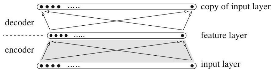
Figure 10.21: Autoencoder for learning the weights of a feature layer. A classical backpropagation network can be used here to learn the identity mapping from the current input layer onto itself. Features form in the hidden layer during learning
