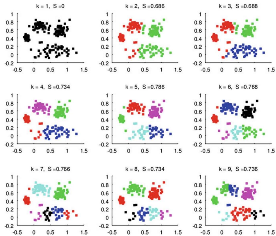
Figure 9.34: Results of the OMRk algorithm for k = 2 to 9 . The best value of S = 0.786 was found with k = 5
