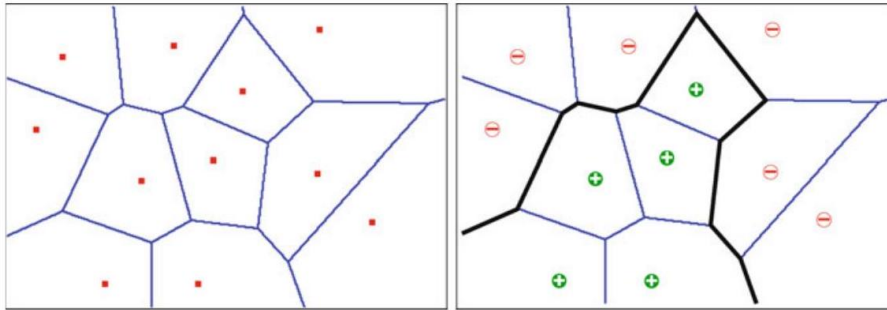
Figure 9.14: A set of points together with their Voronoi-Diagram (left) and the dividing line generated for the two classes M_+ and M_-
