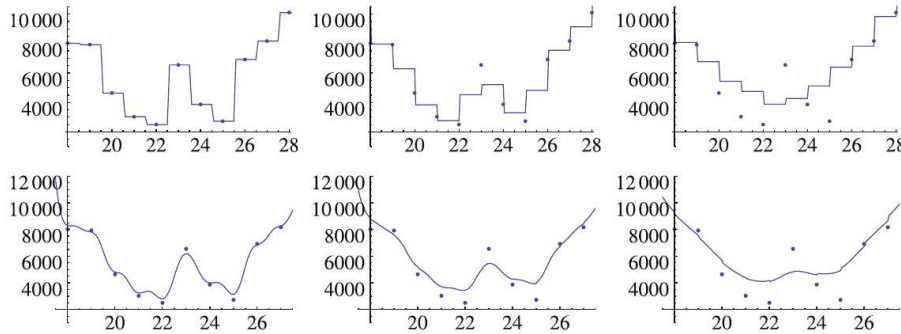
Figure 9.18: Comparison of the k -nearest neighbor method (upper row) with k = 1 (left), k = 2 (middle) and k = 6 (right), to its distance weighted variant (lower row) with \alpha = 20 (left), \alpha = 4 (middle) and \alpha = 1 (right) on a one-dimensional dataset
