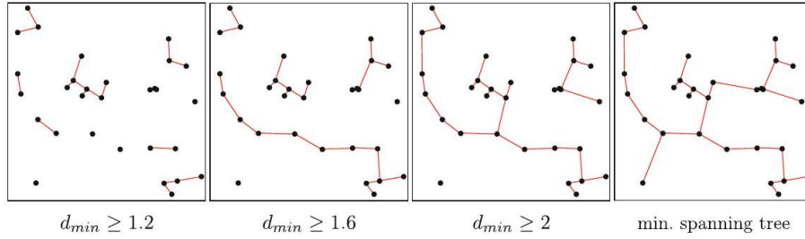
Figure 9.33: In hierarchical clustering, the two clusters with the smallest distance are combined in each step
