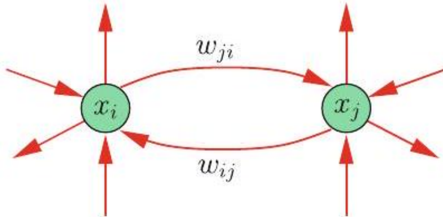
Figure 10.4: Recurrent connections between two neurons in a Hopfield network
