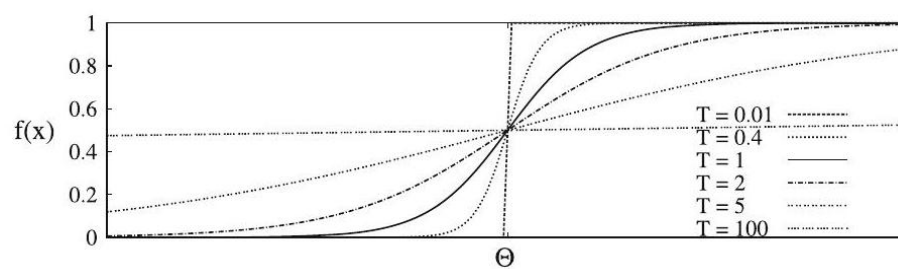
Figure 10.3: The neuron with a step function works like a perceptron with a threshold
