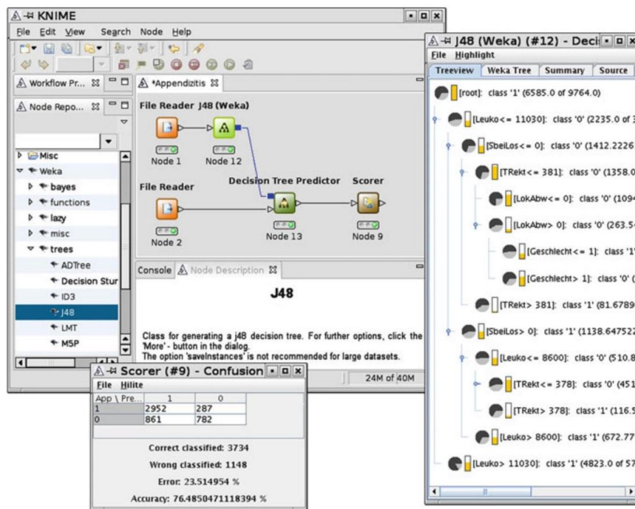
Figure 9.36: The KNIME user interface with two additional views, which show the decision tree and the confusion matrix
