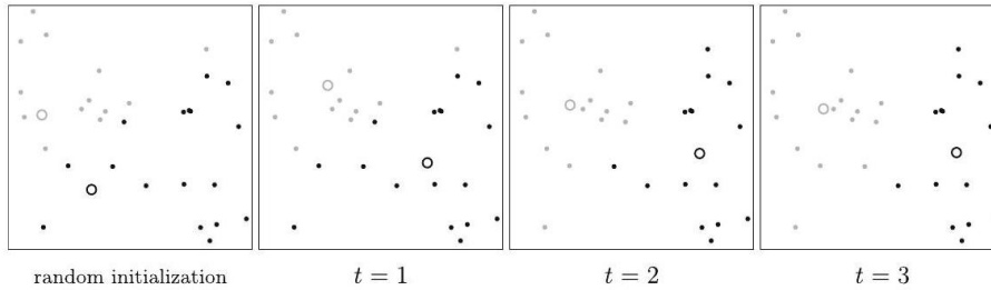
Figure 9.31: k-means with two classes ( k = 2 ) applied to 30 data points. Far left is the dataset with the initial centers, and to the right is the cluster after each iteration. After three iterations convergence is reached
