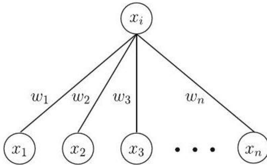
Figure 10.2: The structure of a formal neuron, which applies the activation function f to the weighted sum of all inputs
