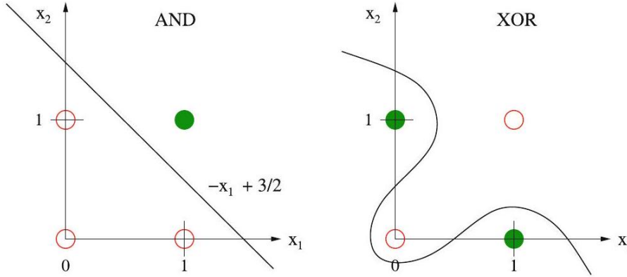
Figure 9.8: The boolean function AND is linearly separable, but XOR is not ( 0 \hat{=} true, 0 \hat{=} false)
