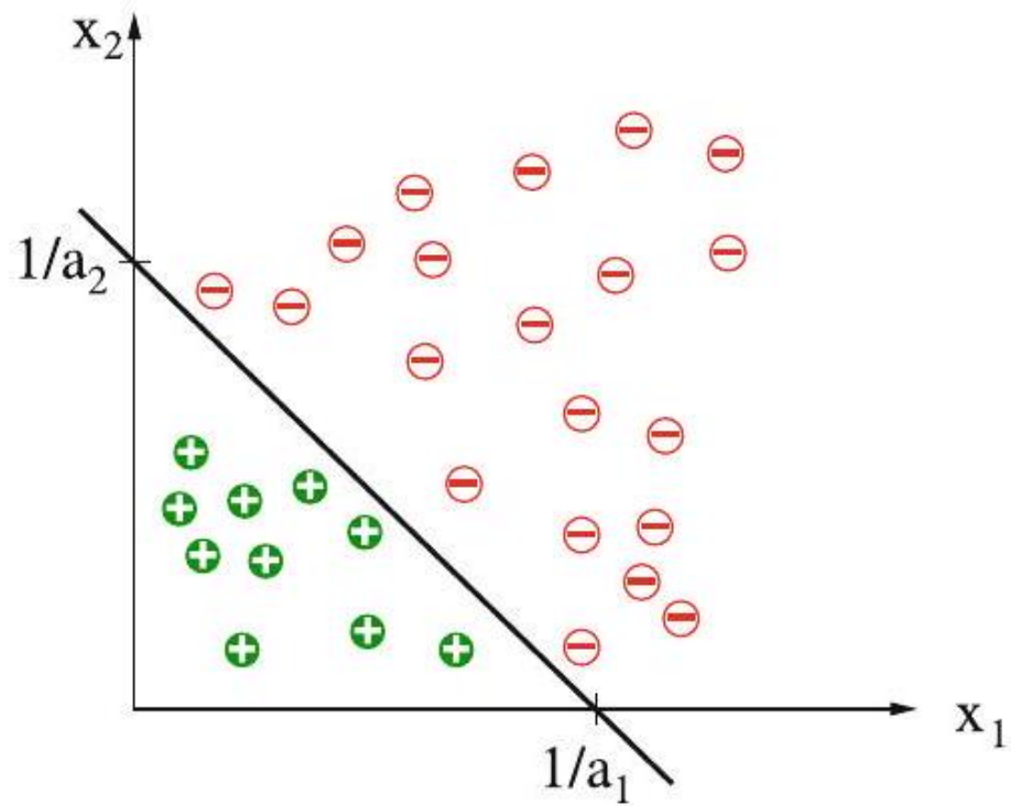
Figure 9.7: A linearly separable two dimensional data set. The equation for the dividing straight line is a_1x_1 + a_2x_2 = 1
