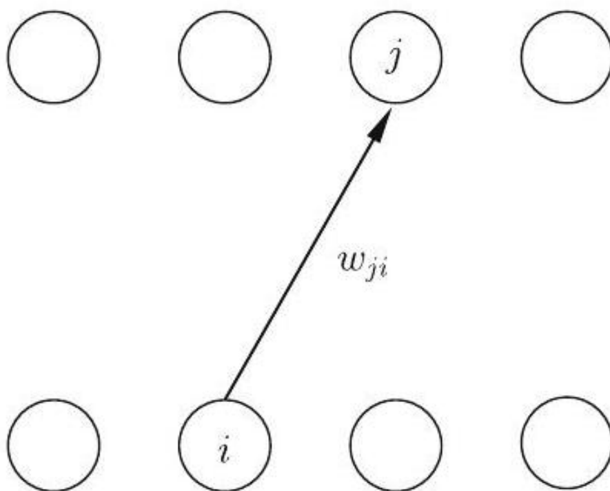
Figure 10.14: Designation of the neurons and weights for the application of the backpropagation rule
